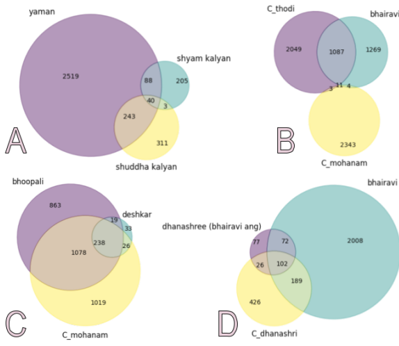
Figure 3: Venn diagrams for sets of raga "words"
