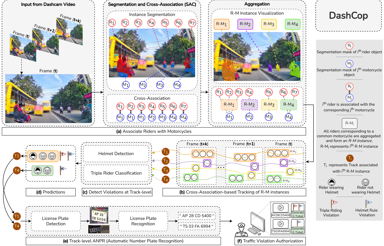
Figure 3. Our Method: (a) Dashcam video frames are input to our Segmentation and Cross-Association (SAC) module, which associates riders with their motorcycles to form rider-motorcycle (R-M) instances. (b) These R-M instances are then fed into a cross-association-based tracker, which robustly tracks them across frames and outputs track information T_i for each R-M instance R-M_i . (c) This track information is used by the violation module to predict triple riding and helmet rule violations. (d) In the illustration, R-M instance R-M_1 is flagged for both triple riding (red flag) and helmet rule violations, while R-M_4 is flagged for a helmet rule violation (blue flag). (e) The track information T_1 and T_4 , corresponding to R-M_1 and R-M_4 respectively, are fed into the ANPR module, which detects and reads the license plates. (f) Finally, the generated E-ticket, with supporting evidence, is shared with traffic authorities for authorization.
