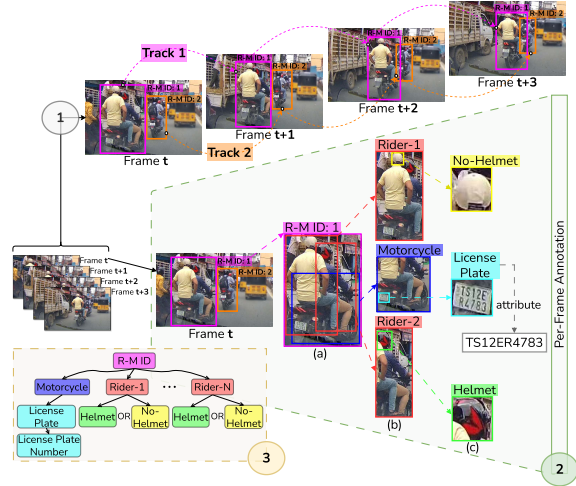
Figure 2. Annotation schema for our RideSafe-400 dataset. Refer to Sec. 3 for details.
